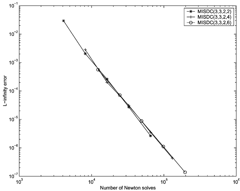
Fig. 11. Log–log plot of L_\infty error versus number of Newton solves for u . Notations are the same as for Fig. 8.
